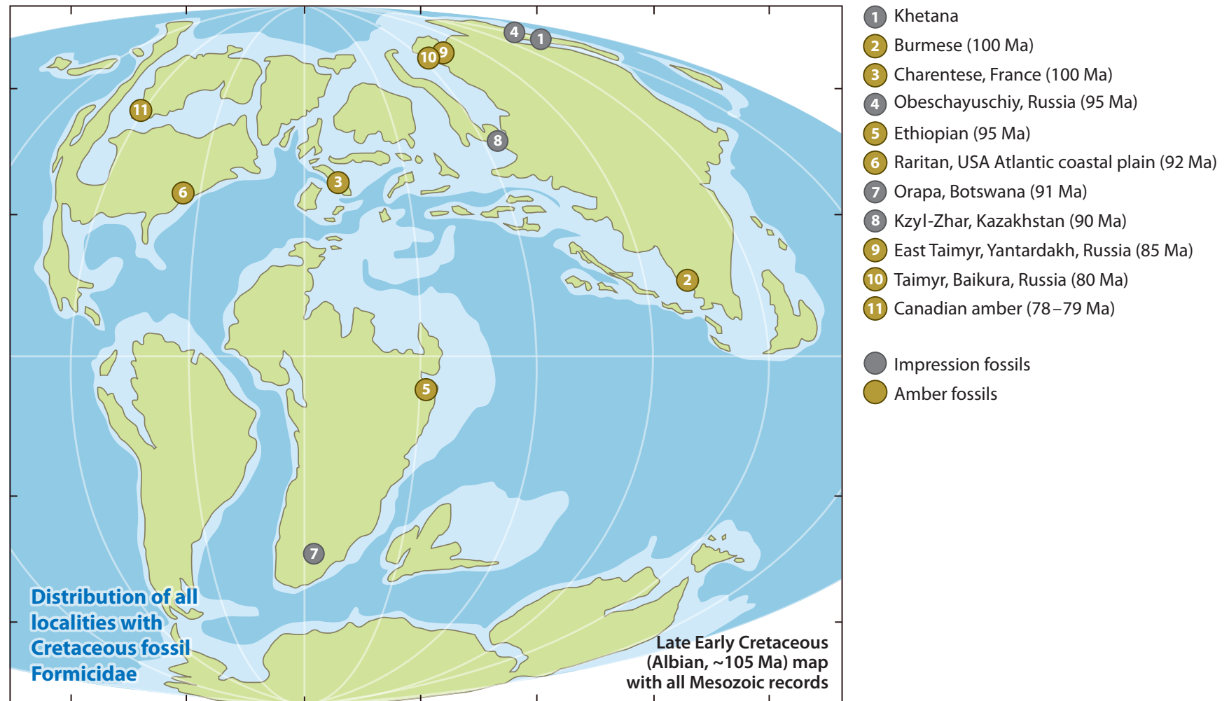
Supplemental Figure 1. Distribution of all Cretaceous localities with fossil Formicidae (maps modified from Blakey RC. 2011. Library of Paleogeography, Colorado Plateau Geosystems, Inc. Mollweide Globes, Late Early Cretaceous (105 mya). http://cpgeosystems.com/105moll.jpg .
