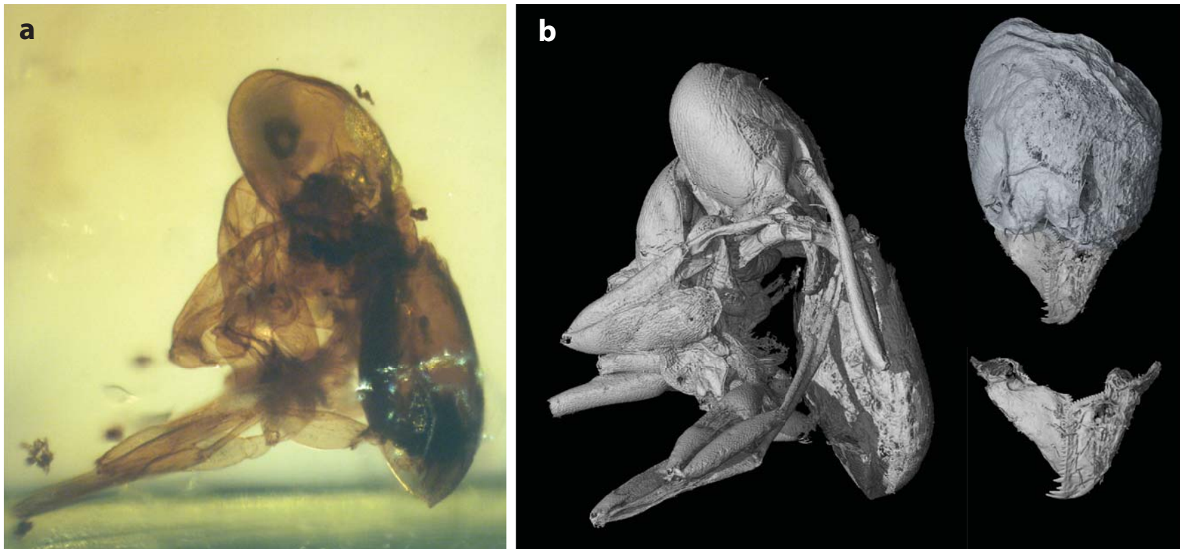
Supplemental Figure 5. (a) A worker ant from 95 Myo amber of Ethiopia. The fossil is curled, which made the observation of many diagnostic features and thus the identification impossible using conventional light microscopes. (b) Three-dimensional virtual reconstruction in phase contrast synchrotron microtomography, followed by a virtual dissection, allows access to all morphological features, as detailed here with the head and mandibles, and identification of a Dolichoderinae (taxon currently under study). Images courtesy of V. Perrichot/C. Soriano/P. Tafforeau/ESRF.
