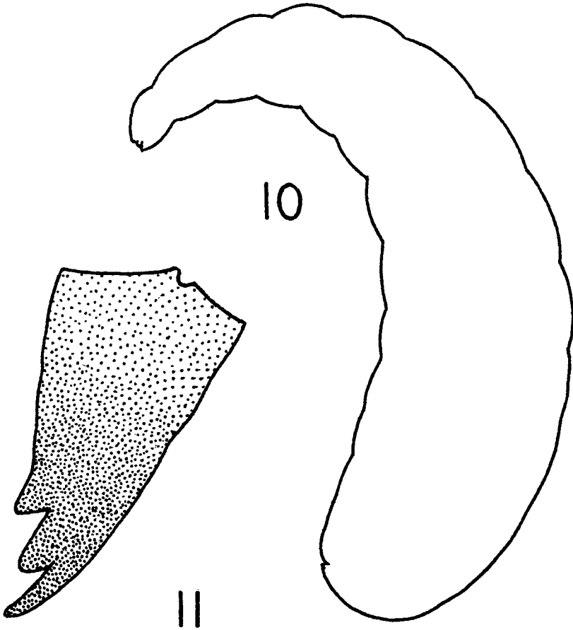
FIG. 10. Myrmeciiform body profile. FIG. 11. Myrmeciiform mandible shape.
